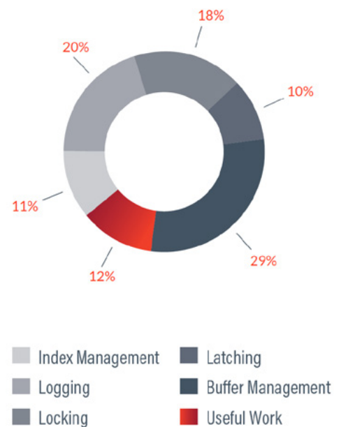
General Purpose RDBMS Processing Profile
